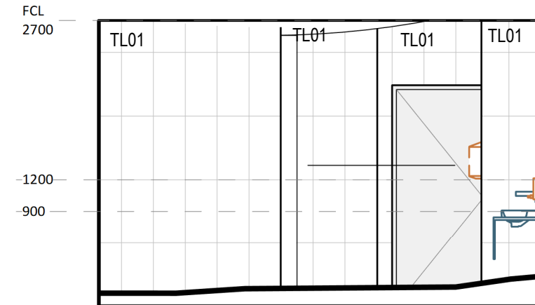
2 ELEVATION DETAIL 60-131 1 : 50
