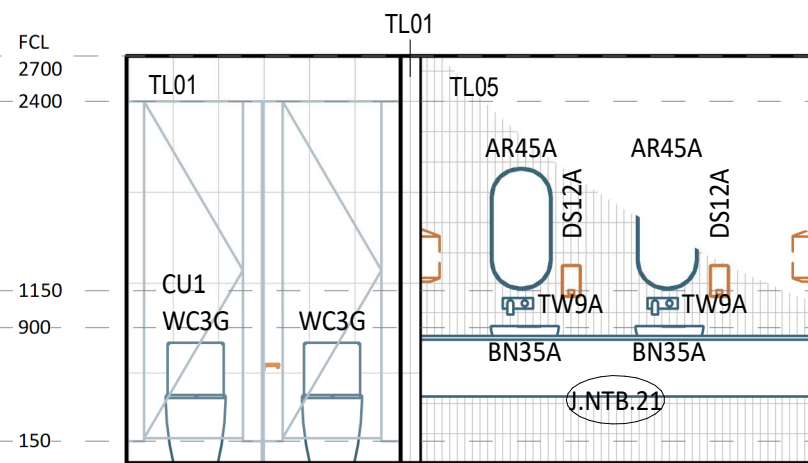
8 ELEVATION DETAIL 60-131 1 : 50
