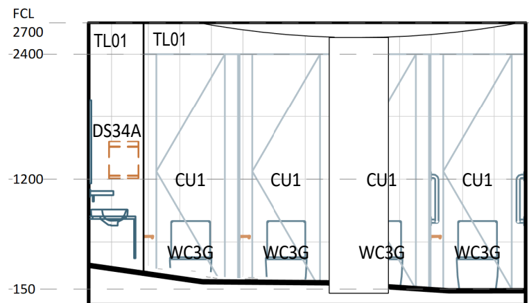
4 ELEVATION DETAIL 60-131 1 : 50
