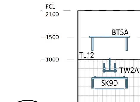
12 ELEVATION DETAIL 60-036 1 : 50
