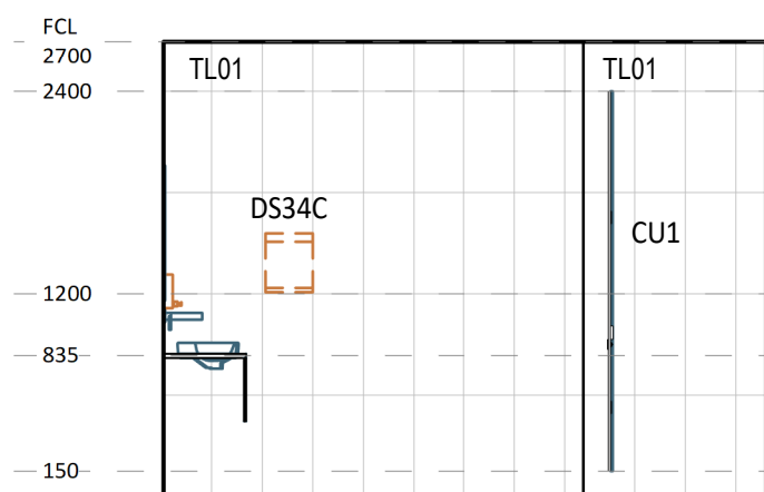
9 ELEVATION DETAIL 60-042 1 : 50
