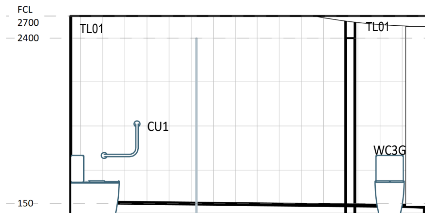
5 ELEVATION DETAIL 60-033 1 : 50
