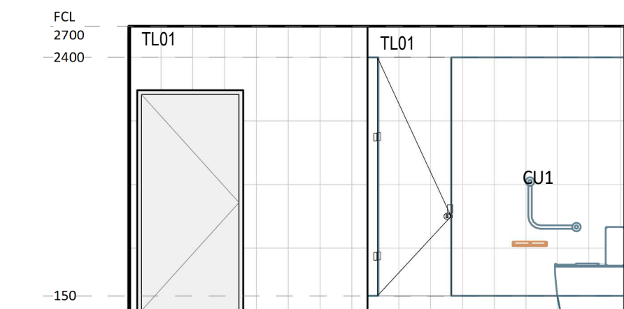
10 ELEVATION DETAIL 60-131 1 : 50
