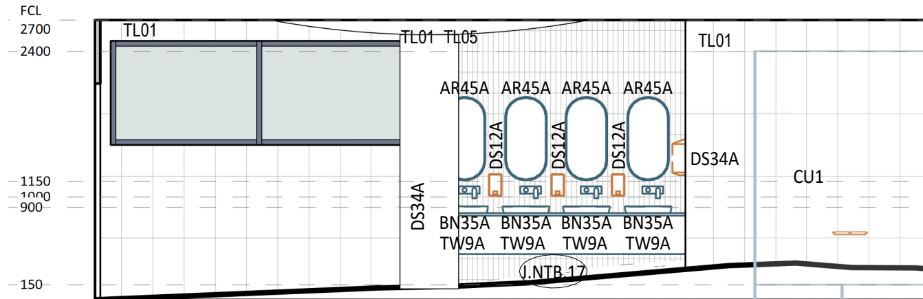
3 ELEVATION DETAIL 60-036 1 : 50
